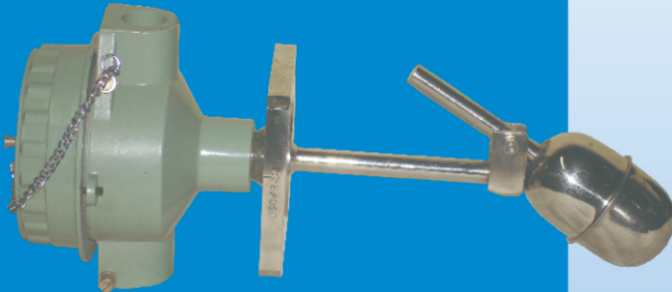
MODEL No. : SMT-04-F82-FLP (FLAME PROOF ENCLOSURE)
